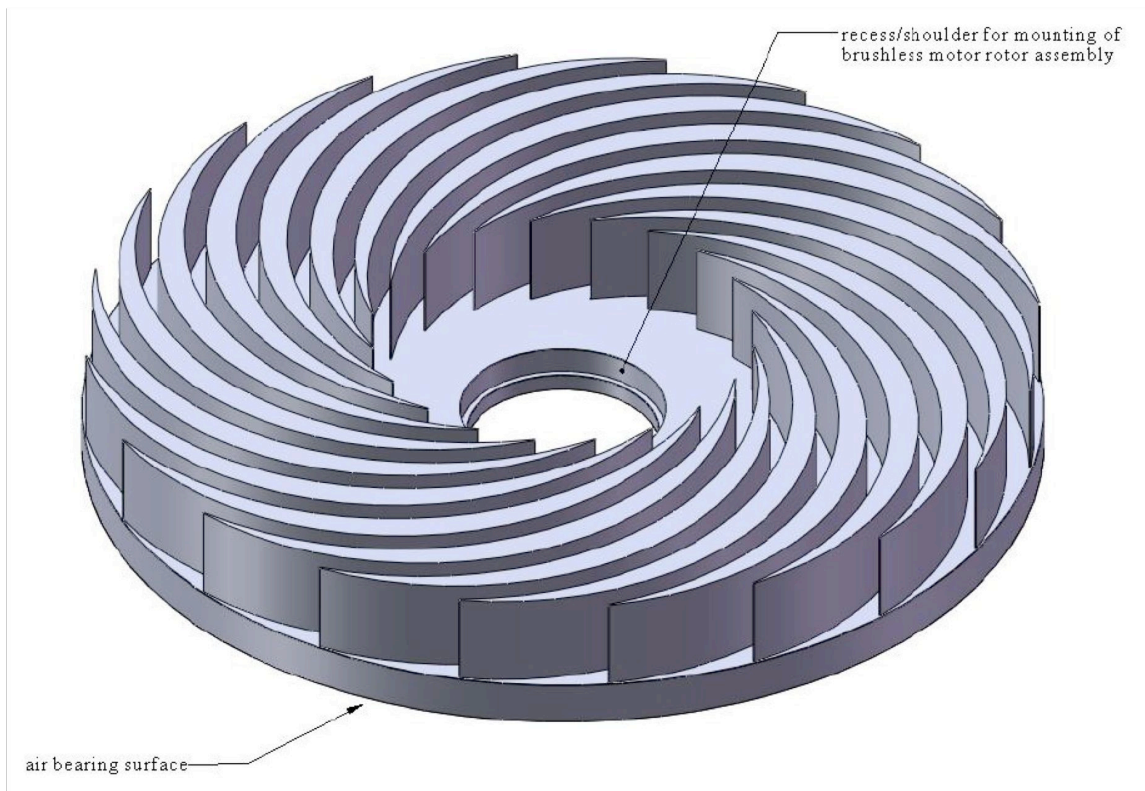
Figure 11b: SolidWorks CAD drawing of heat-sink-impeller. The heat-sink-impeller was CNC machined out of a solid block of 7075 aluminum and anodized black to facilitate the recording of infrared temperature measurements.
