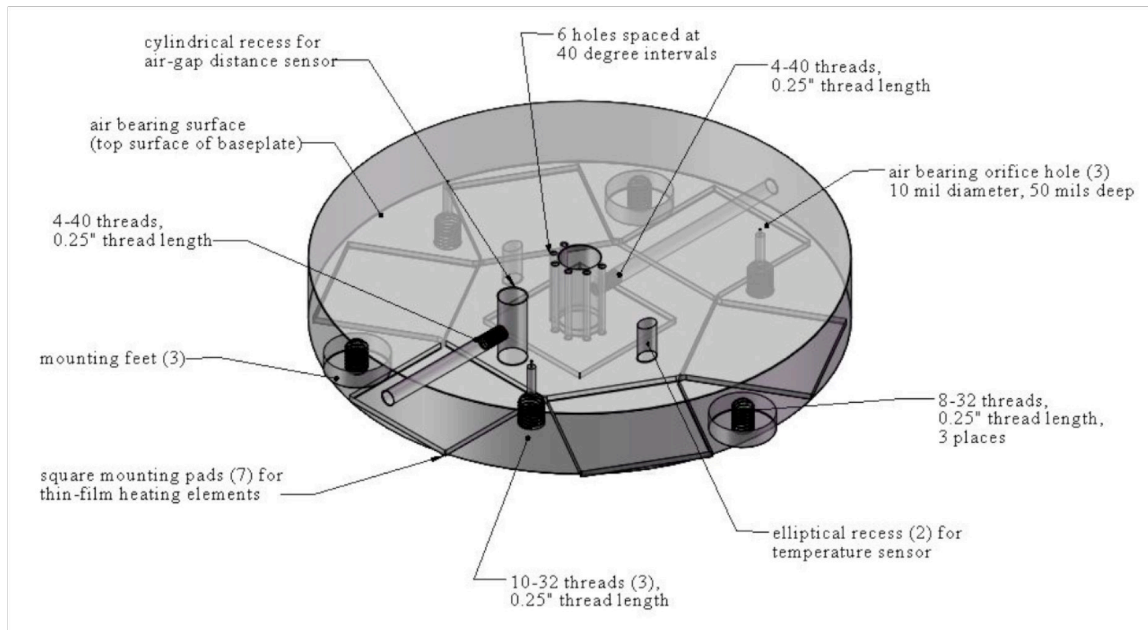
Figure 11a: SolidWorks CAD drawing of air bearing cooler base plate. The base plate was CNC machined out of a solid block of 7075 aluminum and anodized black to facilitate the recording of infrared temperature measurements.
