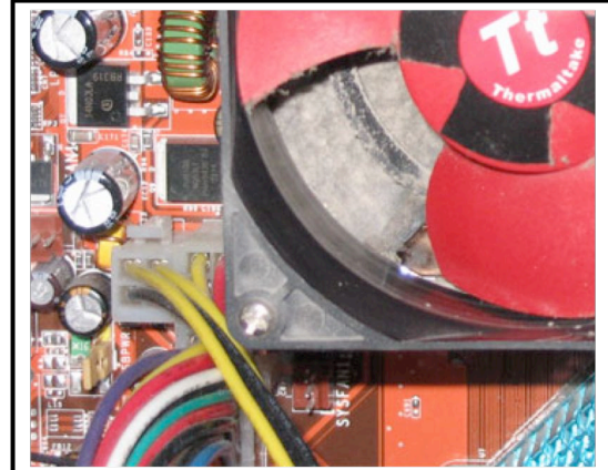
Figure 4: Heat sink fouling in a conventional CPU cooler. The finned heat sink, which is stationary, cannot be seen because it's completely covered in dust. The fan blades, which rotate at several thousand rpm, are nearly dust-free despite operating in the same environment.
