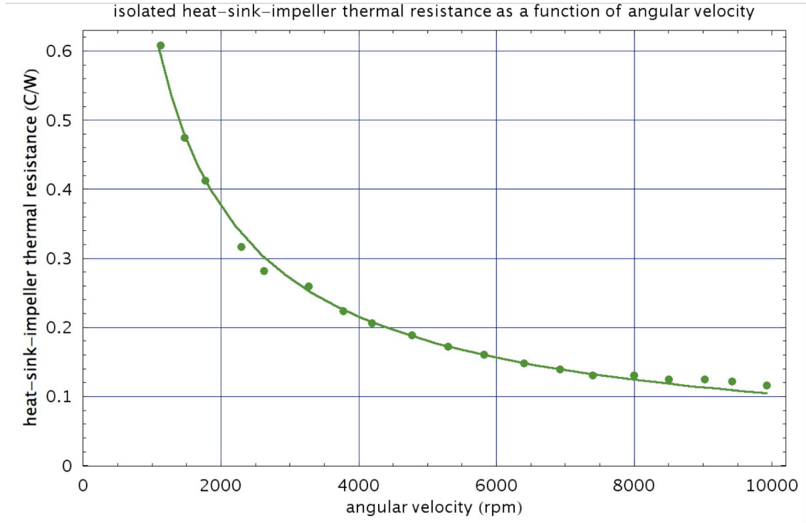
Figure 19: Experimentally measured value of R_{xfer} as a function of angular velocity.
