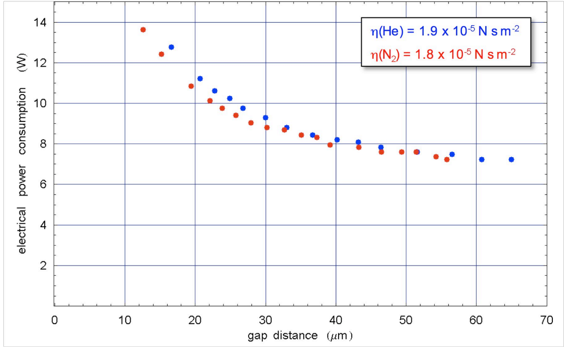
Figure 24: Brushless motor electrical power consumption as a function of air bearing gap distance for \omega = 5000 rpm. The data obtained with nitrogen and helium in the air gap region are nearly identical because the absolute viscosities of He and \text{N}_2 are nearly equal.
