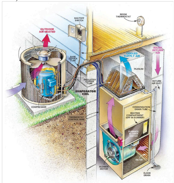
Figure 7: Typical split system residential HVAC installation.
