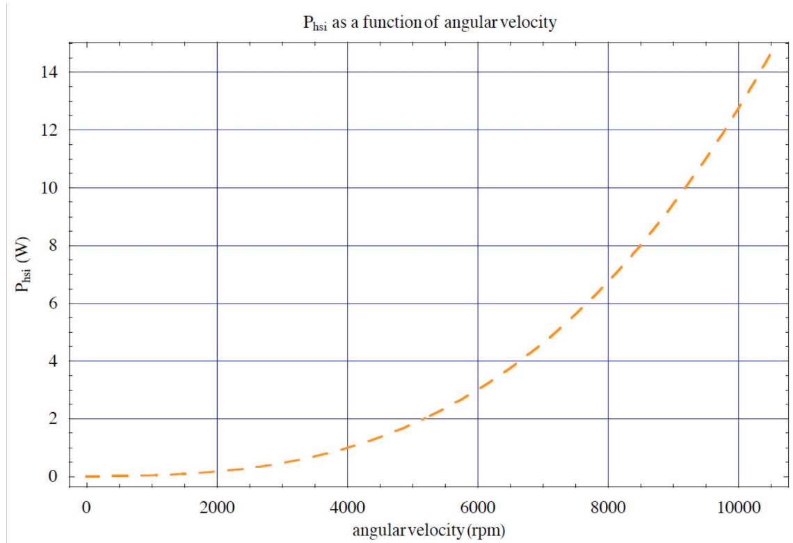
Figure 28: Electrical power consumption associated with rotation of heat-sink-impeller as a function of angular velocity (the effects of air gap shearing friction has been subtracted out).
