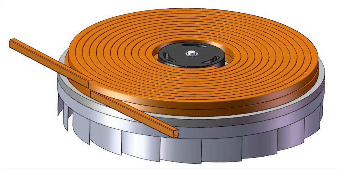
Figure 8: Schematic drawing showing application of air bearing heat exchanger concept to an air conditioner condenser. Such a unit can be made extremely compact compared to a traditional fan-plus-serpentine-finned-tube architecture, and fouling of the outer surface of the soldered copper tubing assembly has no effect on condenser performance. A second identical air bearing cooler (not shown) can be fused to the opposing face of the soldered copper tubing assembly to lower the thermal resistance of the heat exchanger by an additional factor of 2 if desired. An air conditioner evaporator unit can be implemented in an analogous structure. In the case of the air conditioner evaporator, it is also possible to enclose the heat-sink-impeller assembly in a plenum, such that it also serves to circulate air through the HVAC air duct system.
